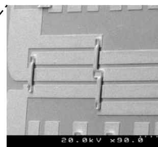
Details of Lange Coupler with printed air-bridges
