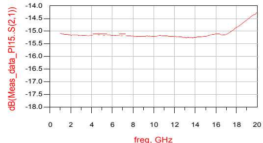
Pad 15 dB, measured data
