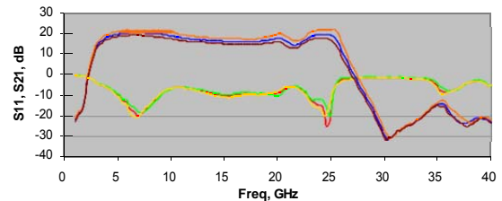
Test results of mounted SMD broadband amplifier 6 to 20 GHz
