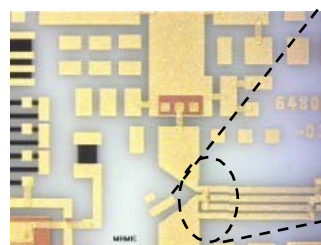
Details of Lange Coupler with printed air-bridges
