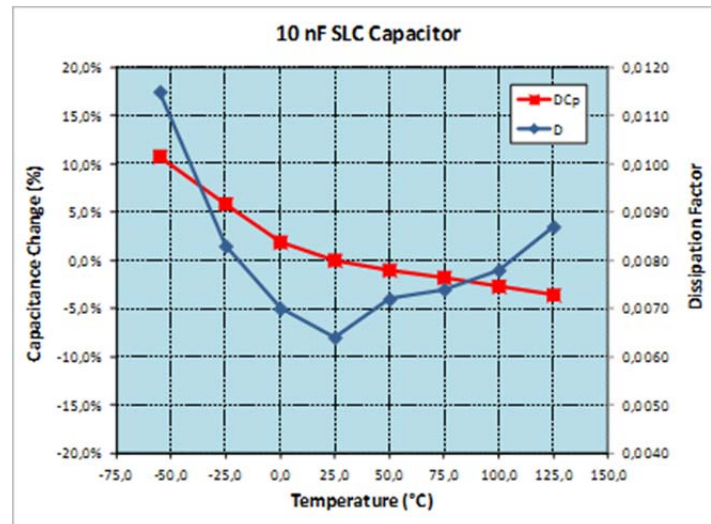
Temperature characteristics
