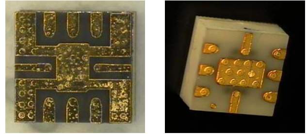
Two different bottom side contact layouts with capped and filled via holes.
